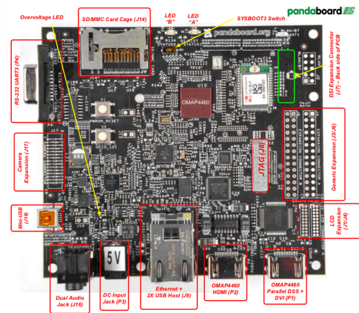
Figure 4.1: Pandaboard
